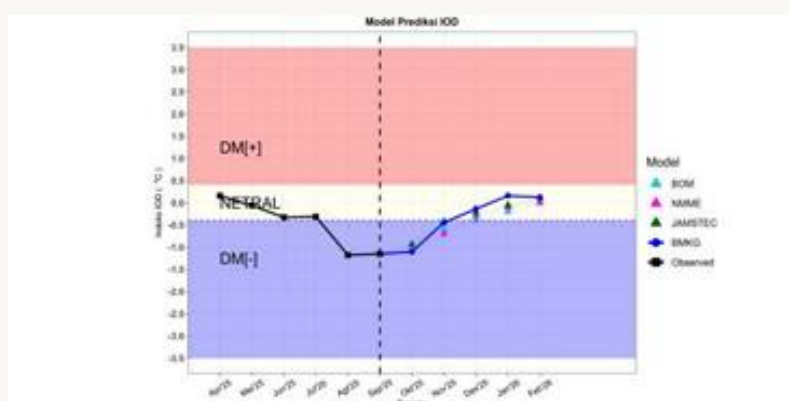
Gambar 2.1.1.C Prediksi Indian Ocean Dipole (IOD)
