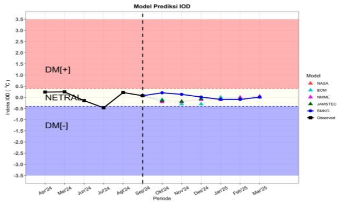
Gambar. 2.2.3 Prediksi Anomali IOD
