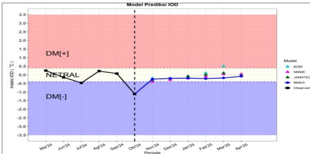
Gambar. 2.2.3 Prediksi Anomali IOD
