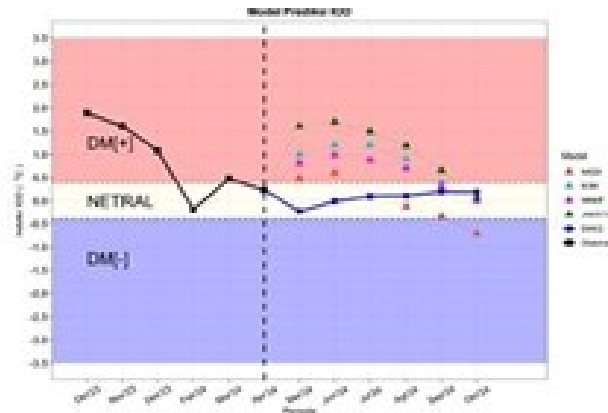
Gambar. 2.2.3 Prediksi Anomali IOD
