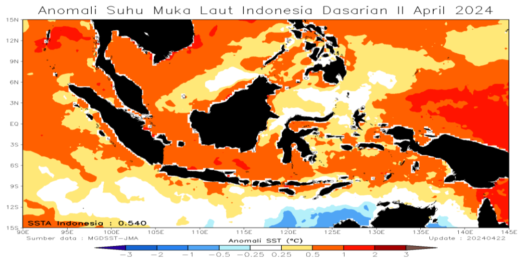
Gambar 1.2.3 SST Bulan April 2024
