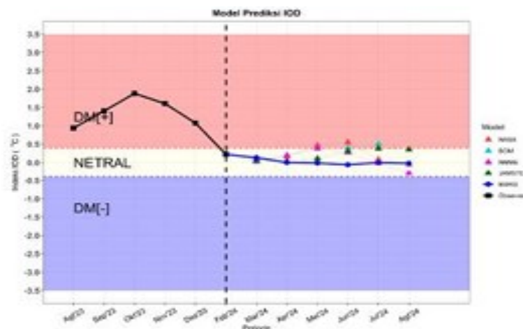
Gambar. 2.2.3 Prediksi Anomali IOD
