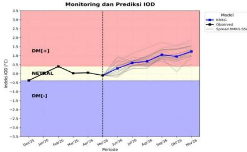
Gambar. 2.2.3 Prediksi Anomali IOD
