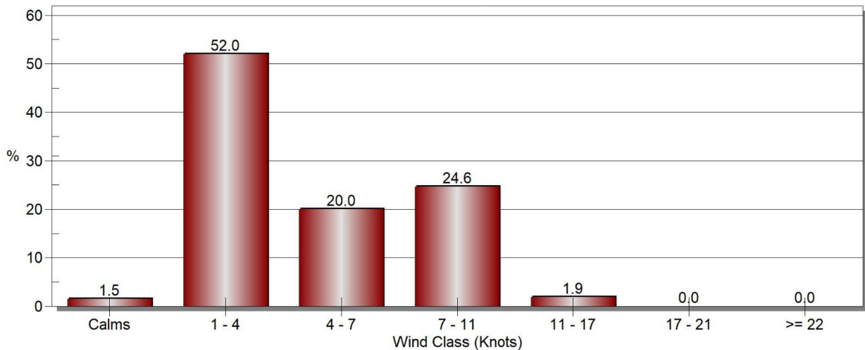
Wind Class Frequency Distribution
