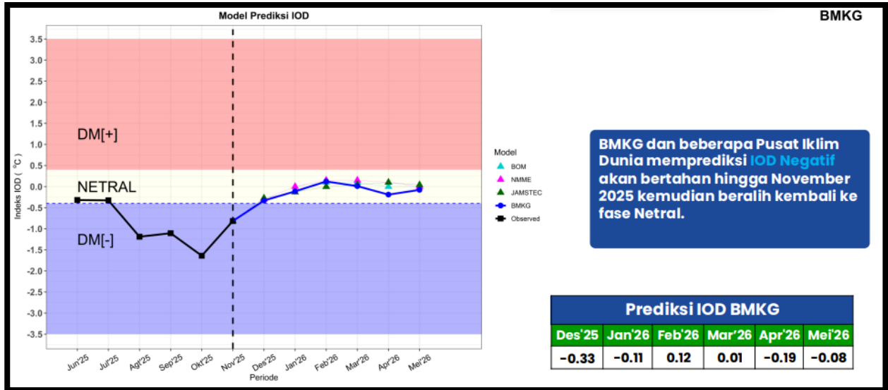
Gambar. 2.2.3 Prediksi Anomali IOD
