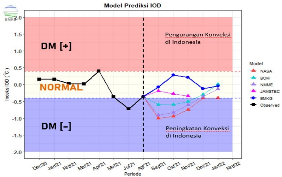
Gambar. 2.2.3 Prediksi Anomali IOD
