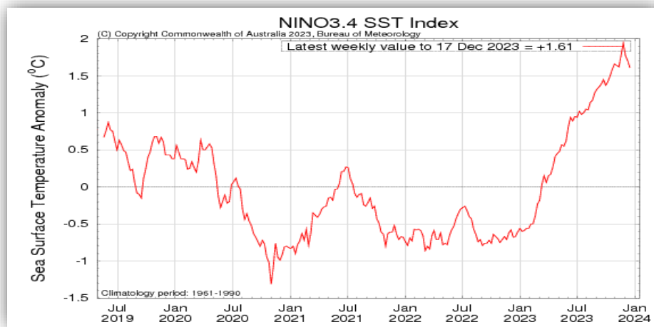
Gambar. 1.2.1 Indeks NINO 3.4 Bulan November 2023
