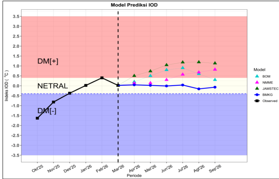
Gambar. 2.2.3 Prediksi Anomali IOD
