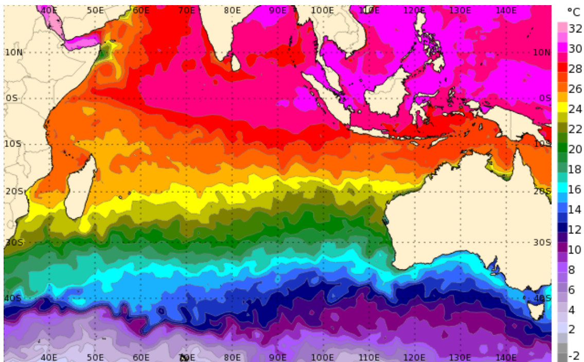
Sea surface temperature (deg C): Daily analysis for Thu 6 Jul 2023 (c) Copyright Australian Bureau of Meteorology | GAMSSA
